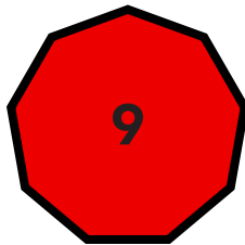
Regular nonagon (enneagon)
