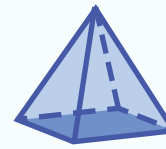
square-based pyramid
