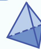
triangular-based pyramid
