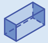
rectangular prism
